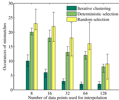
Fig. 6. Comparison of different data point selection strategies
