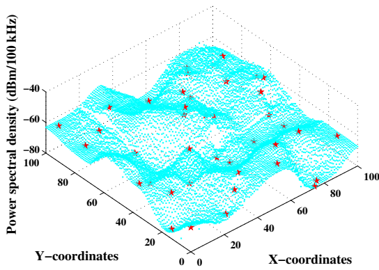
Fig. 2. Estimated power spectral density with 40 sensing locations
