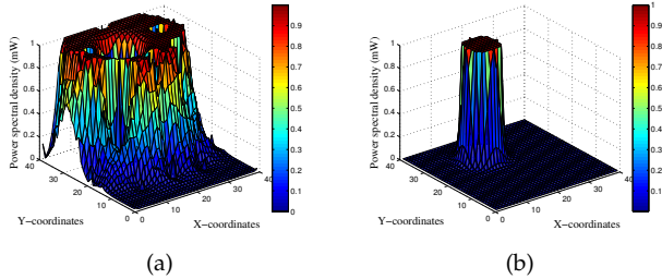
Fig. 16. (a) Estimated and (b) actual signal strengths of a channel in Region 2
