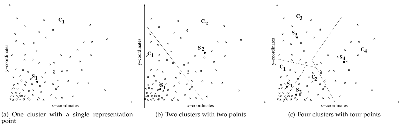
Fig. 4. Iterative clustering and corresponding representation points
