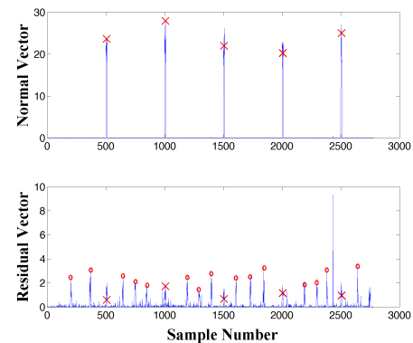
Fig. 6: Measurements of normal space vector squared magnitude ( \|y_{no}\|^2 , upper), and residual space vector squared magnitude ( \|y_{ab}\|^2 , lower) for the synthetic data
