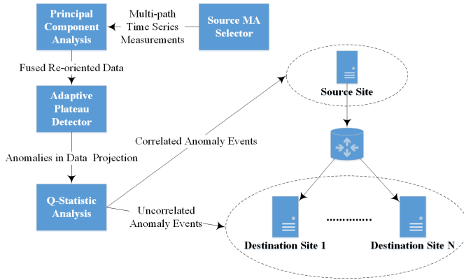
Fig. 4: PCA-APD scheme components diagram
