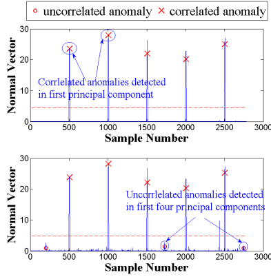
Fig. 7: Measurements of normal space vector squared magnitude \|\mathbf{y}_{no}\|^2 ( \mathbf{P} = [\mathbf{v}_1] , upper) and ( \mathbf{P} = [\mathbf{v}_1, \mathbf{v}_2, \mathbf{v}_3, \mathbf{v}_4] , lower) for the synthetic data
