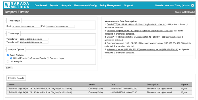
Fig. 13: Narada Metrics Temporal Filter implementation
