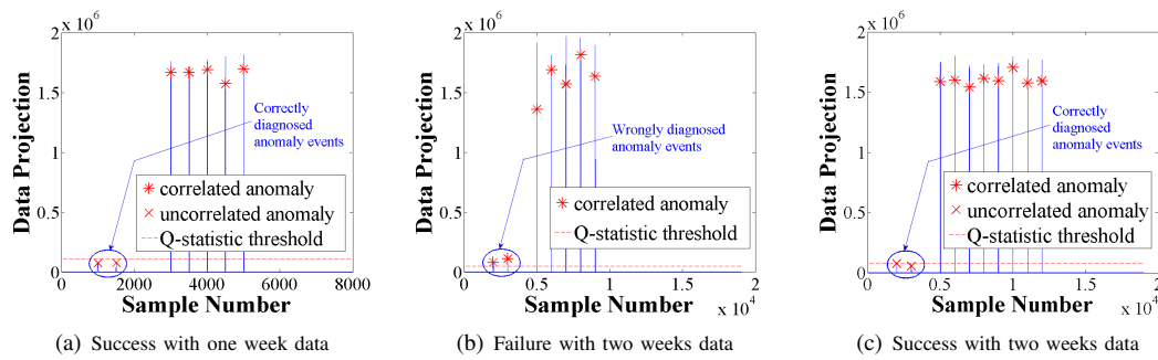
Fig. 19: Accuracy of Q-statistic to successfully isolate correlated and uncorrelated anomaly events for different dataset sizes
