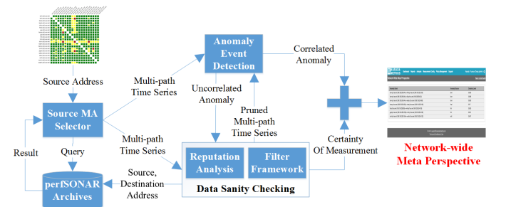
Fig. 3: Schematic diagram of our proposed network-wide anomaly event detection and certainty diagnosis
