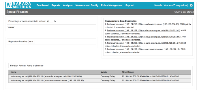
Fig. 14: Narada Metrics Spatial Filter implementation
