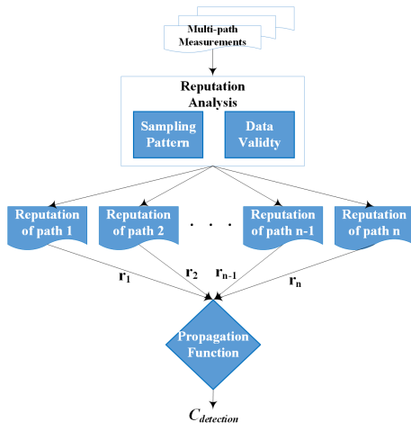
Fig. 8: Reputation-based scheme to evaluate the certainty of a correlated anomaly event detected by PCA-APD-Q-statistic
