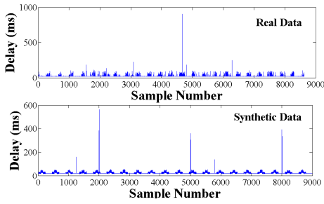
Fig. 15: Data sample comparison between real data and synthetic data
