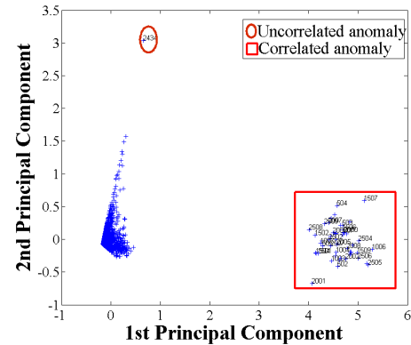
Fig. 5: Correlated and uncorrelated anomaly subspace separation with PCA application
