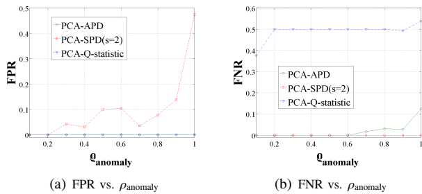
Fig. 17: False alarm rate comparison
